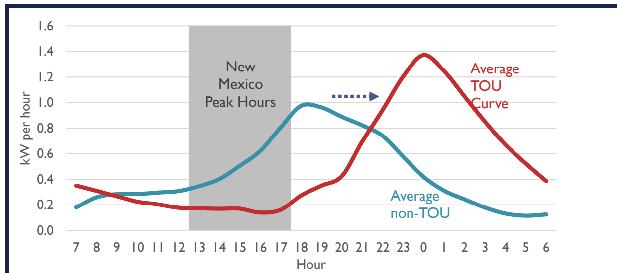
Figure 2. Typical EV charging curve versus the California TOU average EV charging curve, with New Mexico peak hours.
