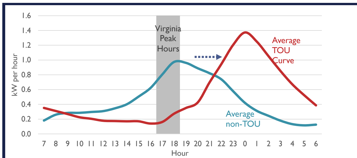
Figure 2. Typical EV charging curve versus the California TOU average EV charging curve, with Virginia peak hours.
