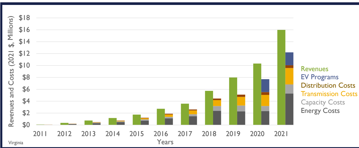
Figure 3. Total costs versus total revenues of EV charging in Virginia per year from 2011-2021.
